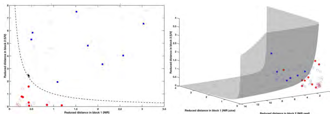
Figure 1 – Illustration of MB SIMCA class space for two (left) and three (right) blocks. The area under the hyperbola/hyperboloid is the acceptance area for the red class.
