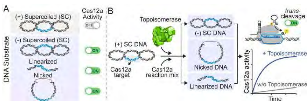
Figure 1. Enzyme-driven switching of DNA topology from positive supercoiling to any relaxed forms enables Cas12a activation that results in a fluorescence output using a Cas12a reaction mix.
