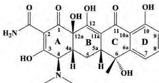
Figure 1. Chemical structure of tetracycline (TC).
