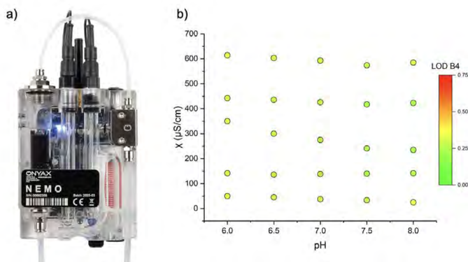
Figure 1. a) OWQM device NEMO, developed by Onyx S.r.l b) Representation of LOD values vs. pH and conductivity.
