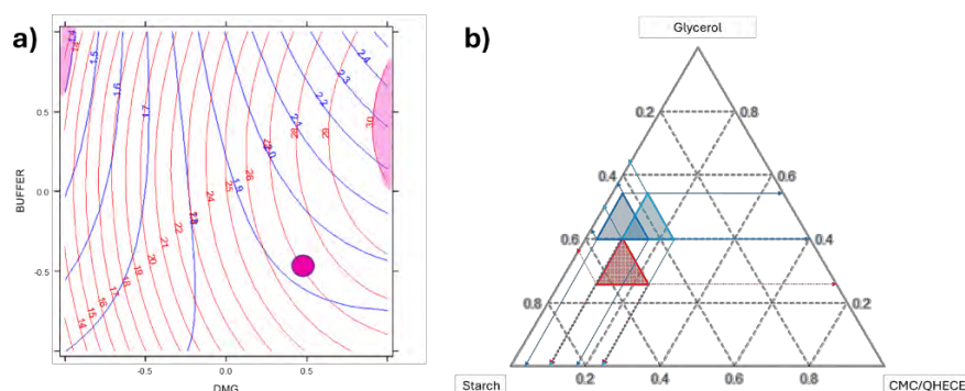
Figure 1. Overlapping FCD isoresponse curves for LOQ and Upper LOQ (a); pseudocomponent domains definition for DMG-BP@ composition optimization (b).
