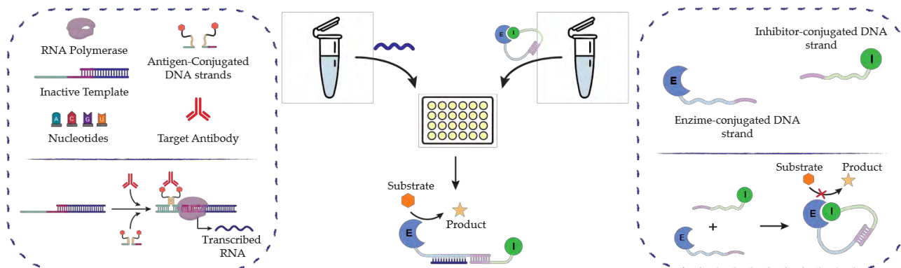
Figure 1. Representative scheme of the platform. (Left) Two proteins conjugated to two different DNA strands with a complementary region (in purple). (Right) The gene network which involves a pair of antigen-conjugated DNA strands designed to hybridize to the single-stranded portion of a synthetic DNA template and reconstitute the incomplete T7 RNA Polymerase promoter domain only upon recognition of a specific target antibody. The transcribed RNA will be able to remove the inhibitor from the enzyme through base pair interactions thus letting the conversion from substrate to product occur.
